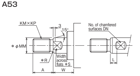
A53 Table of Basic Dimensions
