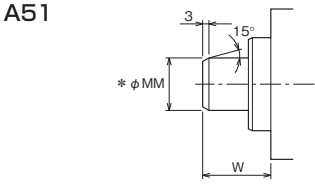
A51 Table of Basic Dimensions
