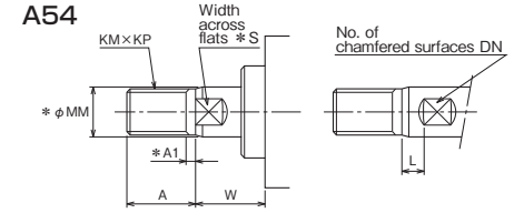
A54 Table of Basic Dimensions
