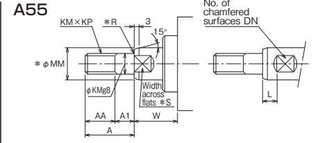
A55 Table of Basic Dimensions
