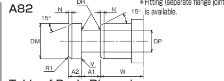
A82 Table of Basic Dimensions
