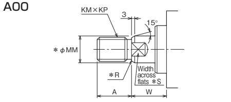
A00 Table of Basic Dimensions (Standard dimensions)
